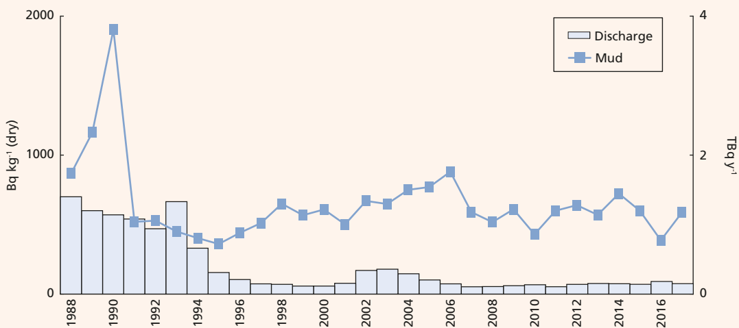
Figure 2.22. Plutonium-alpha liquid discharge from Sellafield and plutonium-239+240 concentration in mud at Ravenglass, 1988-2017
