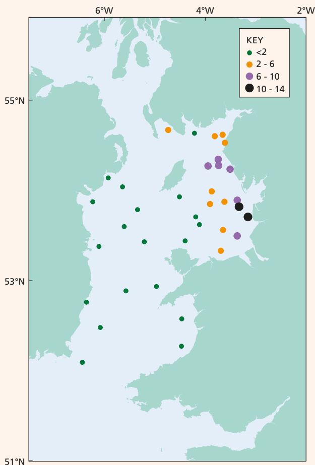
Figure 8.6. Concentrations ( \text{Bq l}^{-1} ) of tritium in surface water from the Irish Sea, August–September 2017
