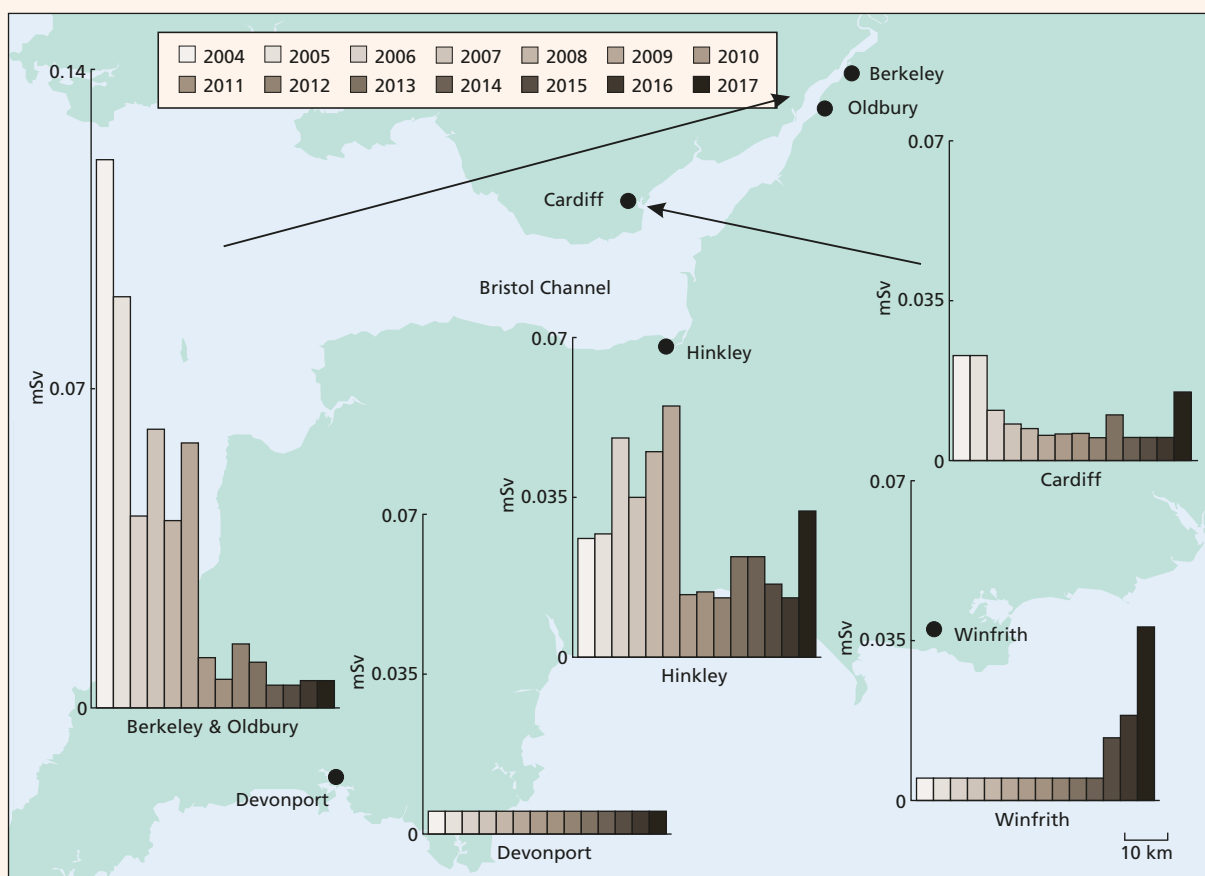
Figure 6.1. Total dose for major sites in the Severn Estuary and south coast, 2004-2017 (Note small doses, less than or equal to 0.005 mSv, are recorded as being 0.005 mSv)
