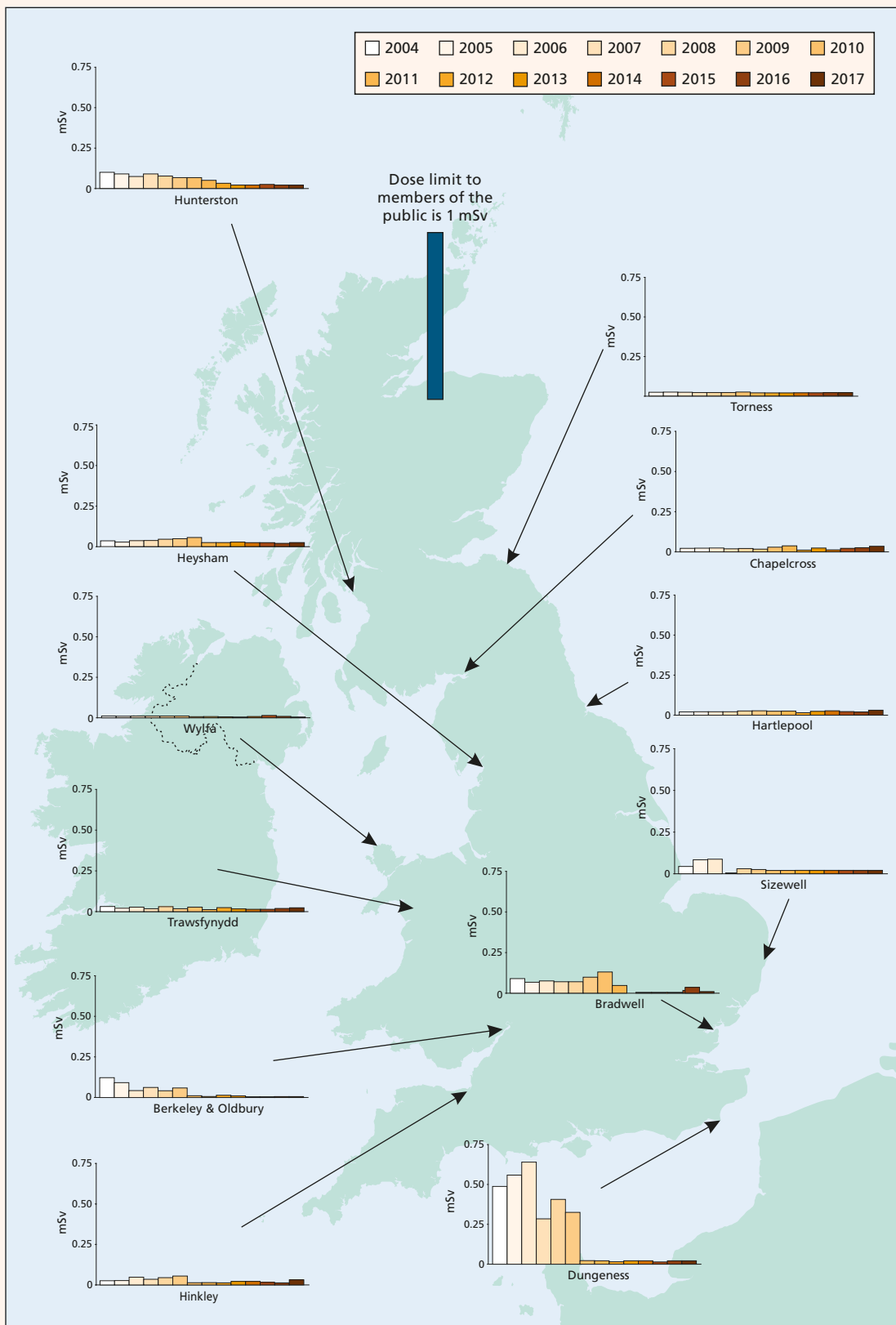
Figure 4.1. Total dose at nuclear power stations, 2004-2017 (Small doses less than or equal to 0.005 mSv are recorded as being 0.005 mSv)
