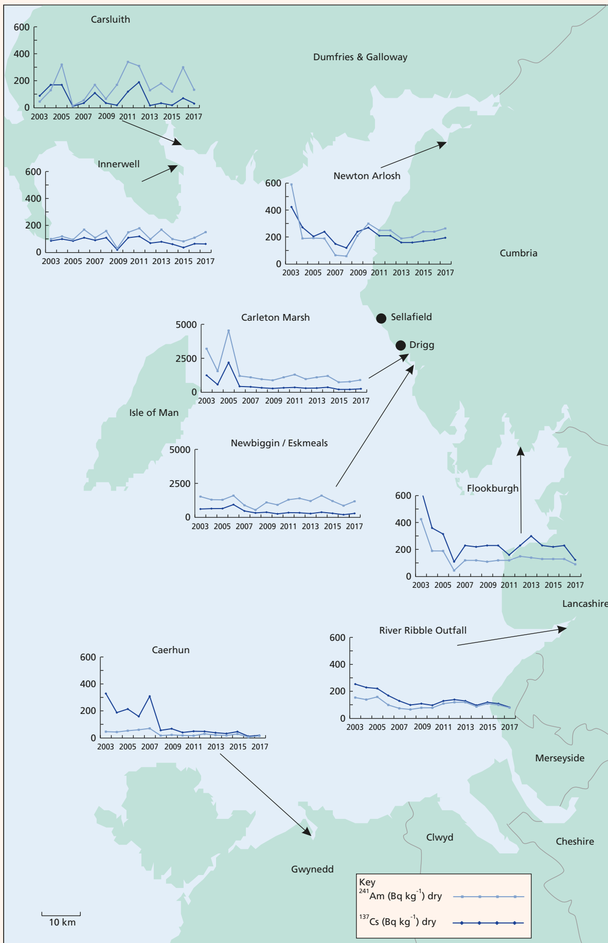
Figure 2.25: Concentrations of americium-241 and caesium-137 in coastal sediments in North West England and South West Scotland between 2003-2017 (Note different scales used for Newbiggin and Carleton Marsh)
