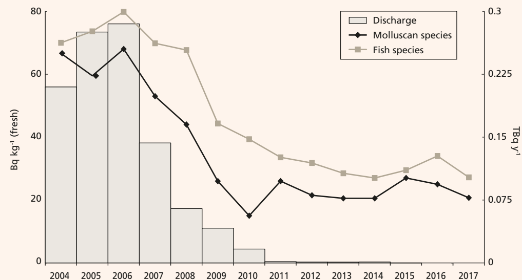
Figure 6.5. Carbon-14 liquid discharge from Cardiff and mean concentrations in fish and molluscs near Cardiff, 2004-2017 (species include all those reported in RIFE for the given year)
