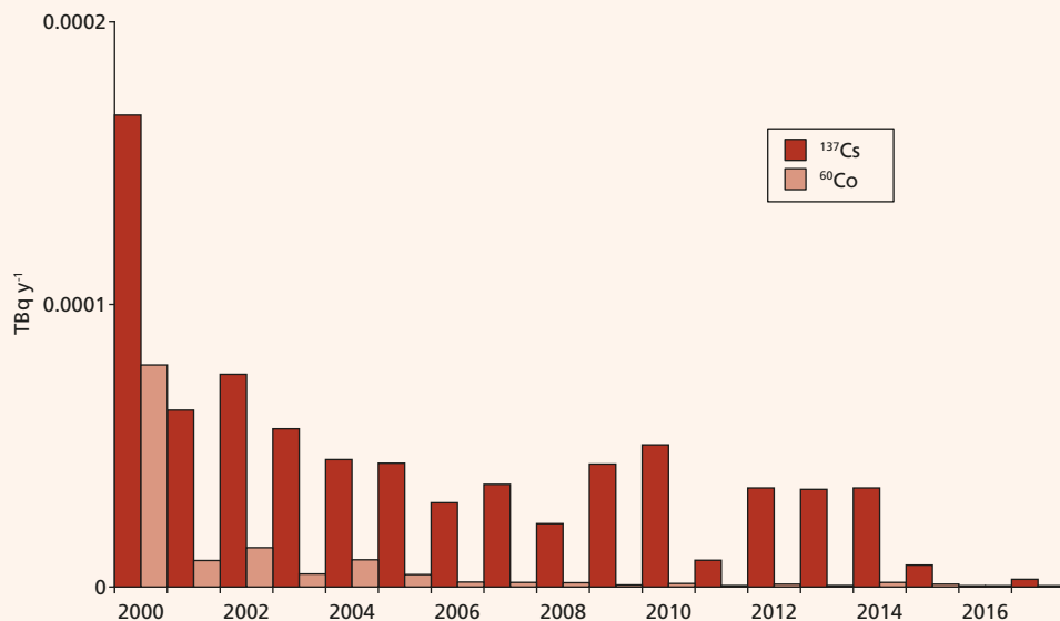
Figure 3.5. Trends in liquid discharges of caesium-137 and cobalt-60 from Harwell, Oxfordshire 2000-2017
