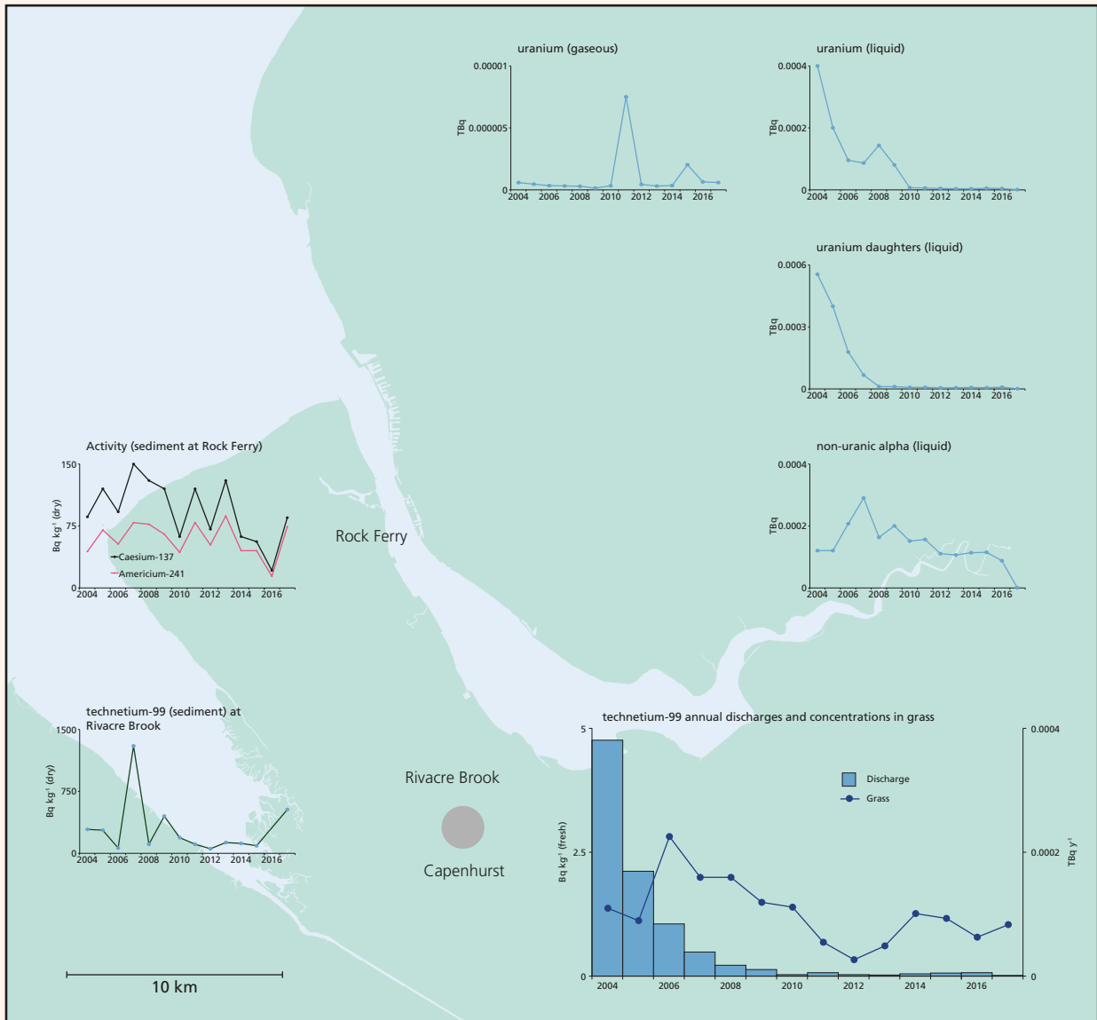
Figure 2.2. Discharges of gaseous and liquid radioactive wastes and monitoring of the environment, Capenhurst (2004-2017) (Note different scales used for discharges and activity concentrations)
