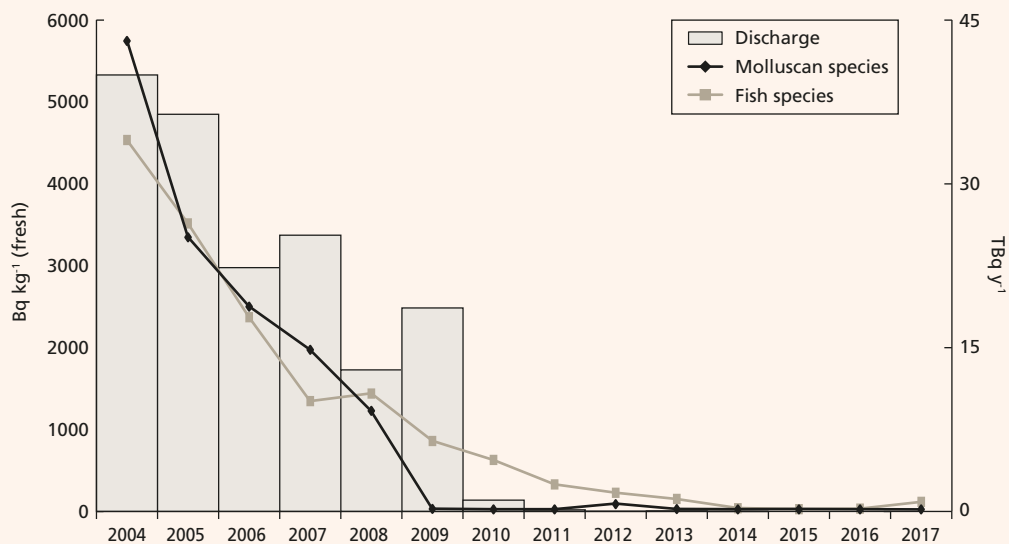
Figure 6.4. Tritium liquid discharge from Cardiff and mean concentrations in fish and molluscs near Cardiff, 2004-2017 (species include all those reported in RIFE for the given year)
