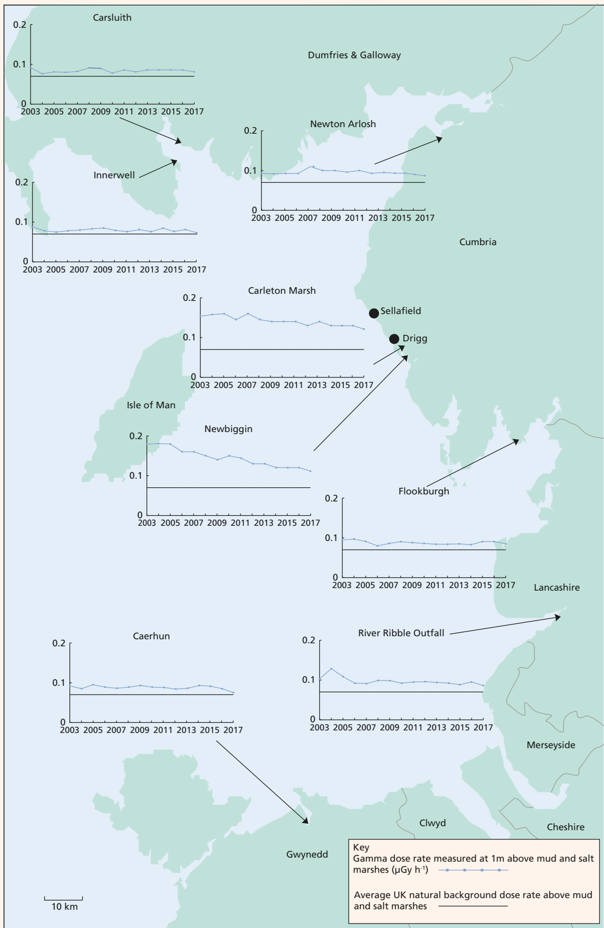
Figure 2.26. Gamma dose rates above fine coastal sediments (mud and salt marshes) in North West England and South West Scotland between 2003-2017
