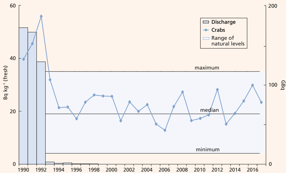
Figure 7.3. Polonium-210 discharge from Whitehaven and concentration in crabs at Parton, 1990-2017
