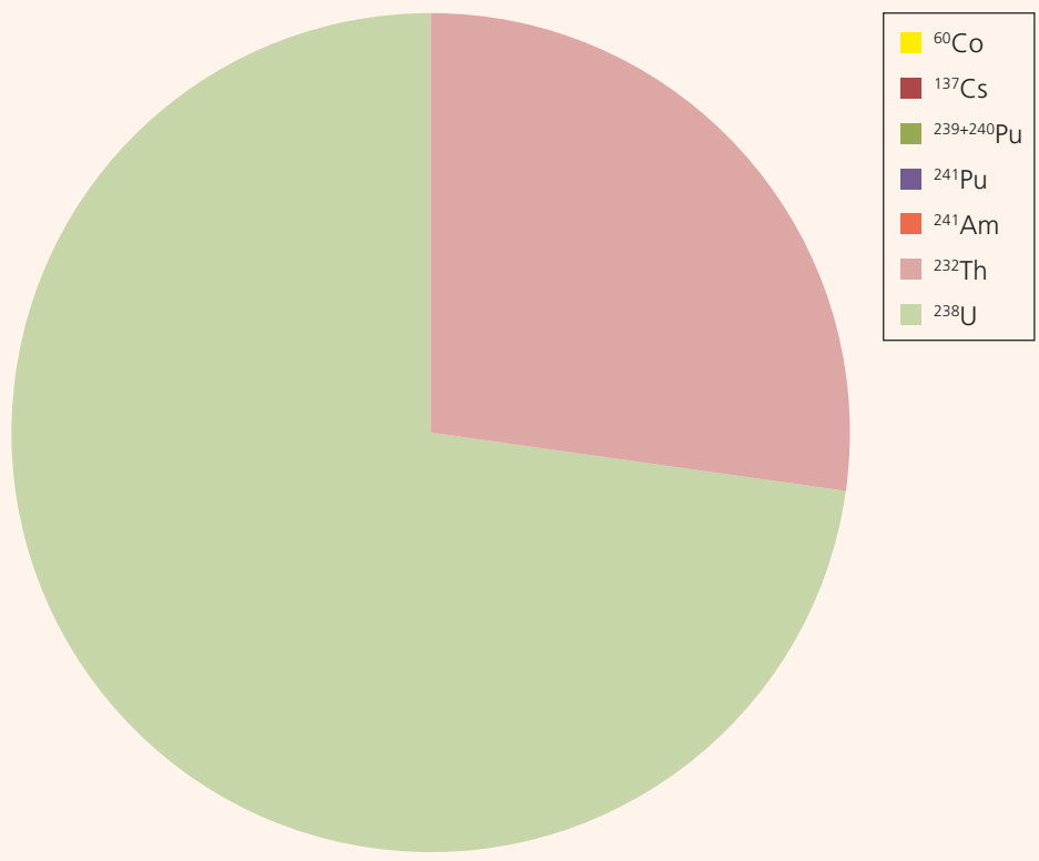
Figure A5.2. Radionuclide contribution to dose to individual members of the public due to dredging Hinkley Point C, Somerset, 2017
