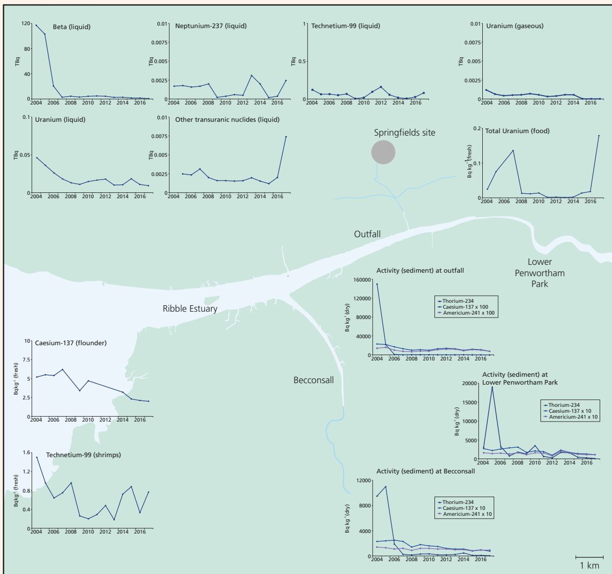
Figure 2.5. Discharges of gaseous and liquid radioactive wastes and monitoring of the environment, Springfields 2004–2017 (Note different scales used for discharges and activity concentrations)
