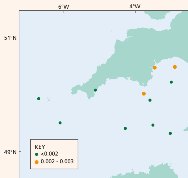
Figure 8.5. Concentrations ( \text{Bq l}^{-1} ) of caesium-137 in filtered surface water from the English Channel, February–March 2017
