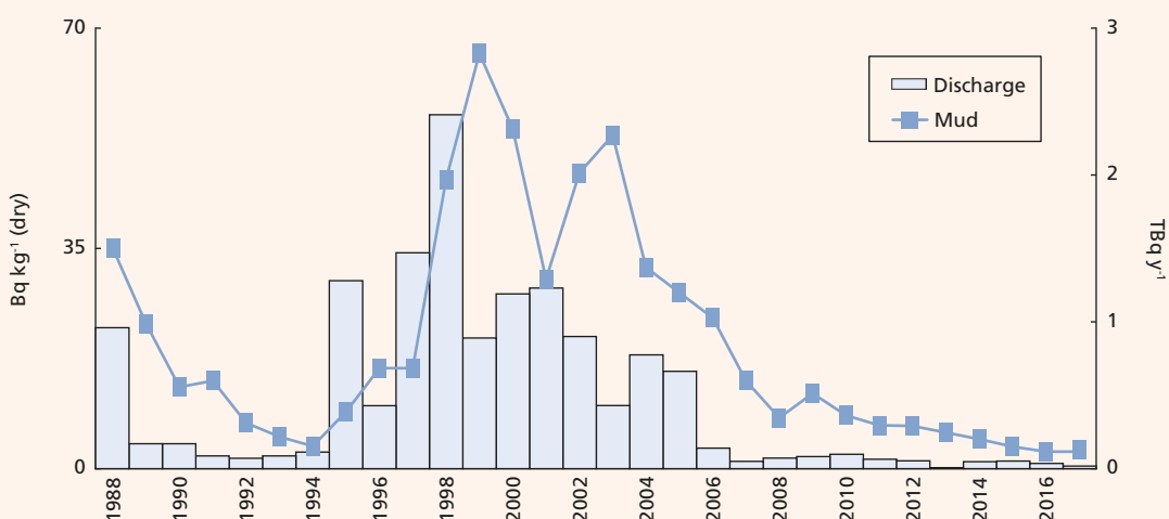
Figure 2.23. Cobalt-60 liquid discharge from Sellafield and concentration in mud at Ravenglass, 1988-2017
