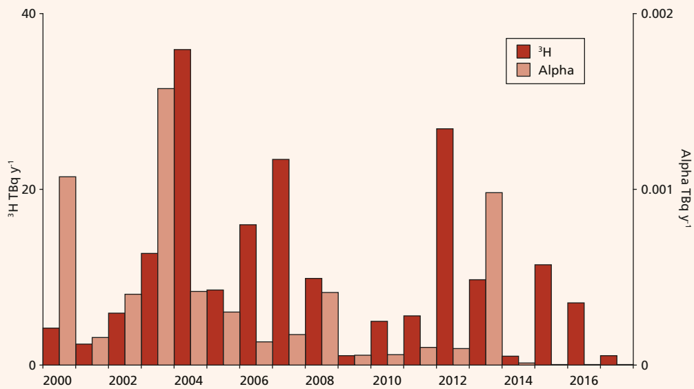
Figure 3.7. Trends in liquid discharges of tritium and alpha emitting radionuclides from Winfrith, Dorset 2000-2017
