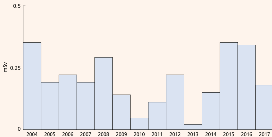
Figure 7.4. Trend in total dose to seafood consumers from naturally-occurring radionuclides near Whitehaven, 2004-2017
