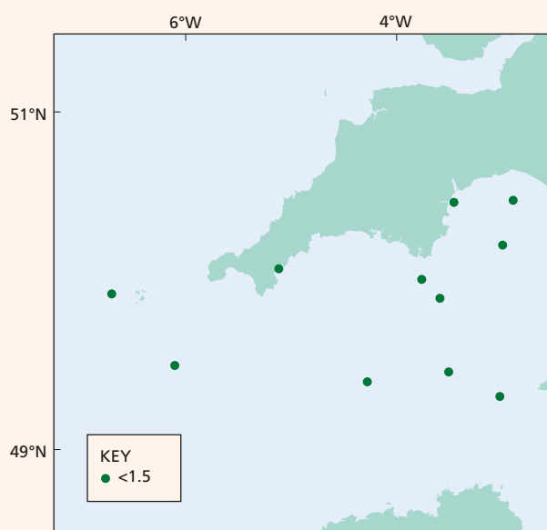
Figure 8.8. Concentrations ( \text{Bq l}^{-1} ) of tritium in surface water from the English Channel, February–March 2017
