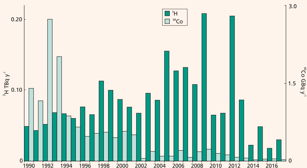
Figure 5.2. Trends in liquid discharges of tritium and cobalt-60 from Devonport, Devon 1990-2017
