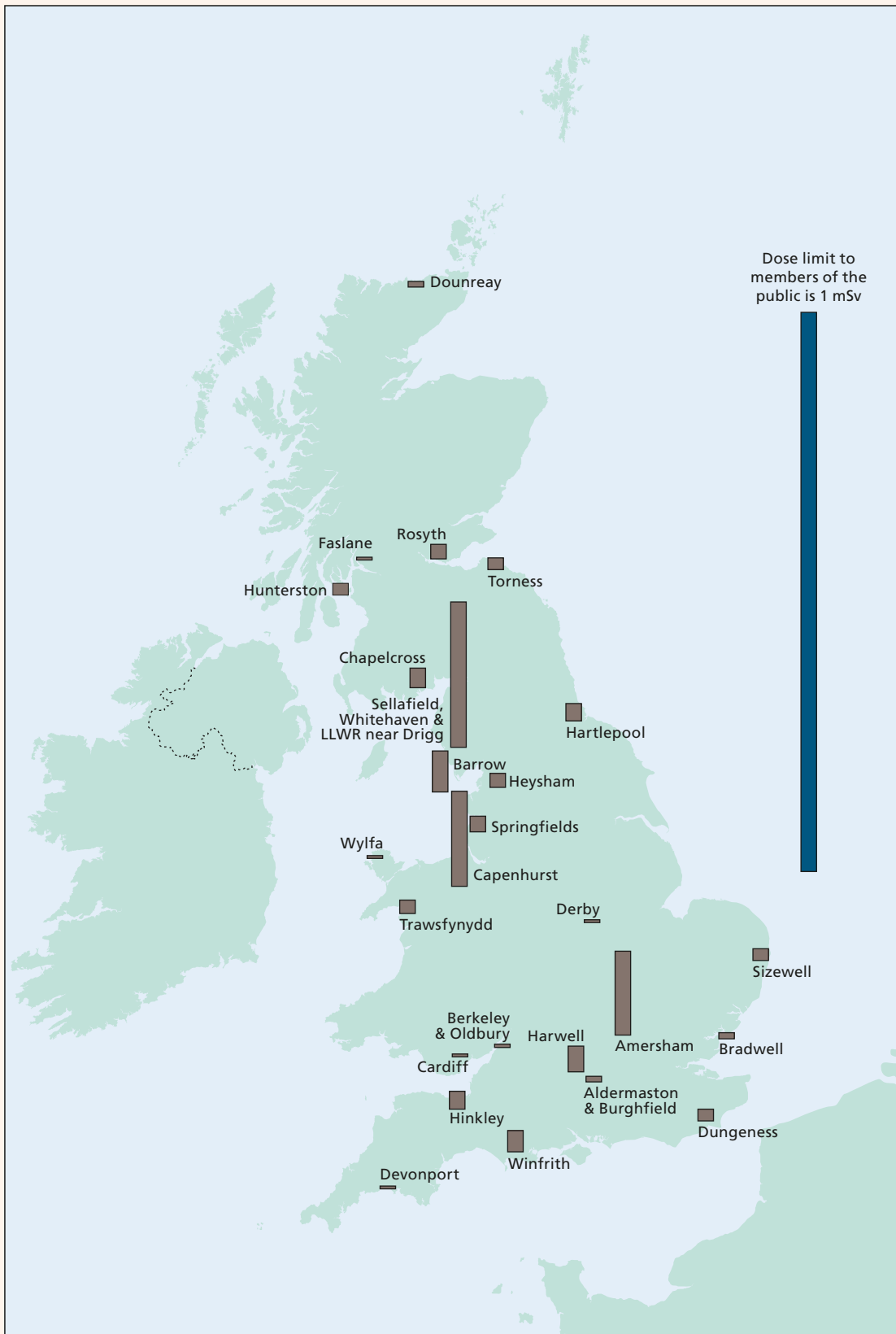
Figure S. Total doses in the UK due to radioactive waste discharges and direct radiation, 2017 (Exposures at Sellafield, Whitehaven and Drigg receive a significant contribution to the dose from technologically enhanced naturally occurring radionuclides from previous non-nuclear industrial operations)
