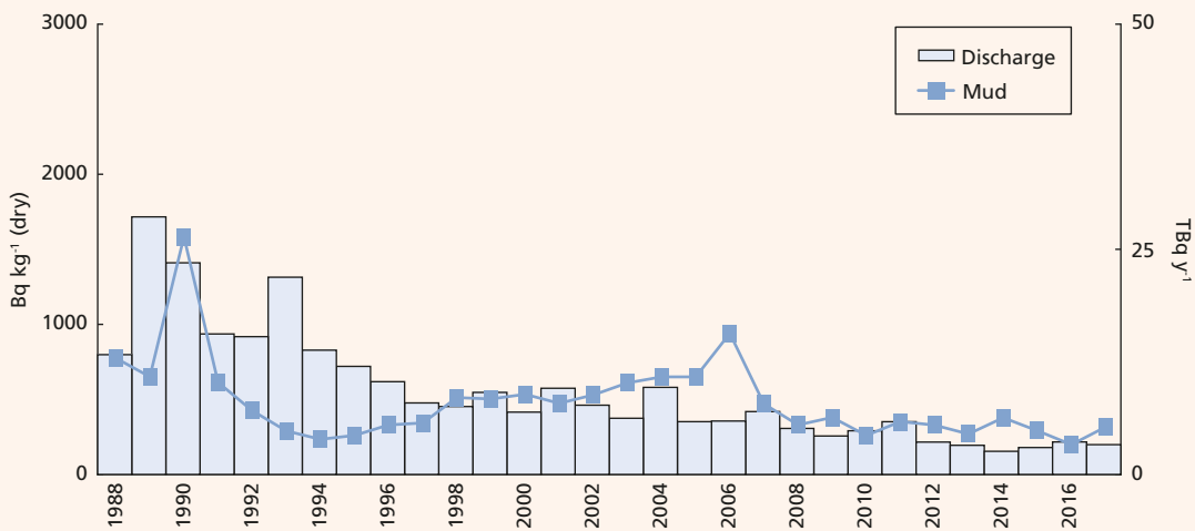
Figure 2.21. Caesium-137 liquid discharge from Sellafield and concentration in mud at Ravenglass, 1988-2017
