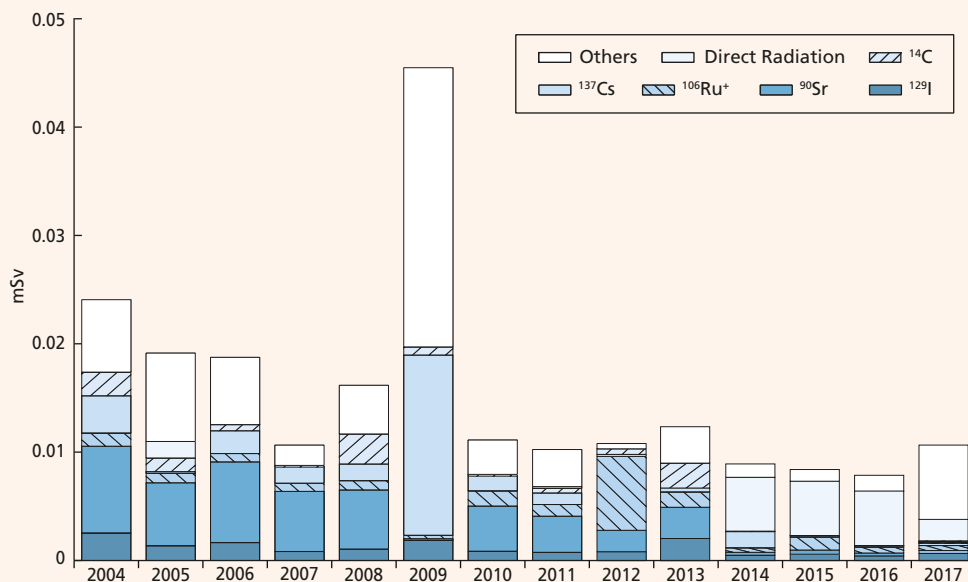
Figure 2.9. Contributions to total dose from gaseous discharge and direct radiation sources at Sellafield, 2004-2017 (+ based on limits of detection for concentrations in foods)
