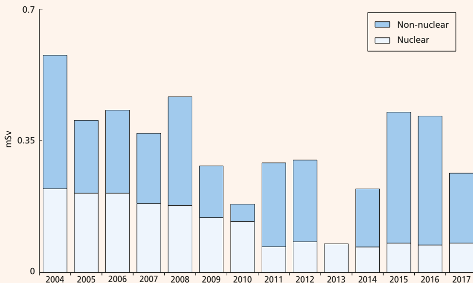
Figure 2.7. Contributions from nuclear and non-nuclear industries to total dose from all sources at Sellafield, 2004-2017 (The highest total dose in 2013 due to Sellafield discharges was to people living on houseboats near Barrow in Cumbria)
