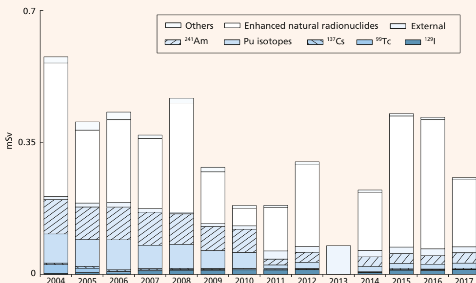
Figure 2.6. Contributions to total dose from all sources at Sellafield, 2004-2017 (The highest total dose in 2013 due to Sellafield discharges was to people living on houseboats near Barrow in Cumbria)
