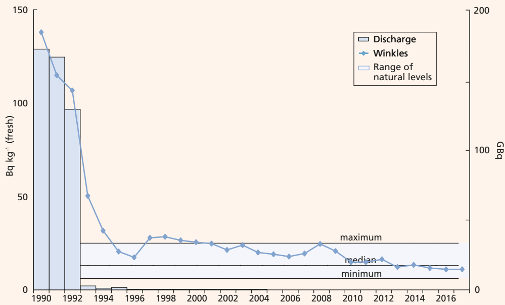
Figure 7.2. Polonium-210 discharge from Whitehaven and concentration in winkles at Parton, 1990-2017
