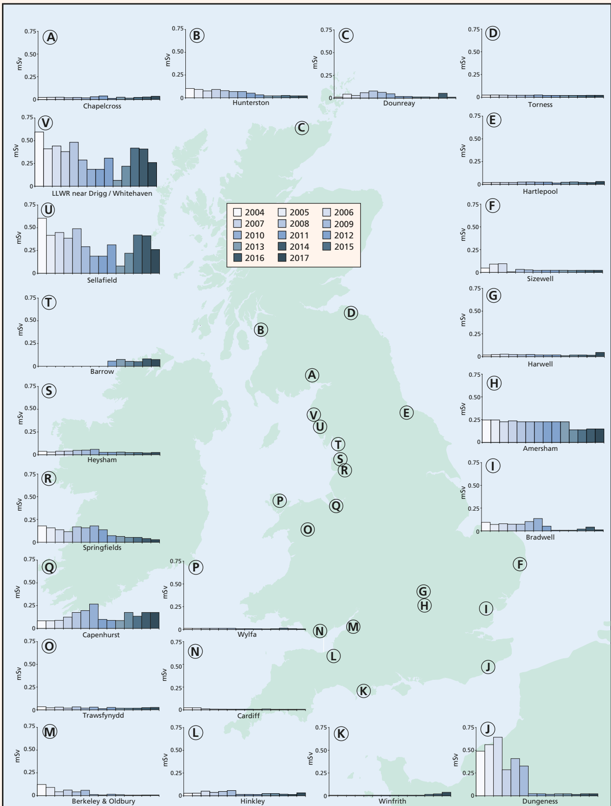
Figure 1.2. Total doses around the UK's nuclear sites due to radioactive waste discharges and direct radiation (2004-2017). (Exposures at Sellafield/Whitehaven/LLWR receive a significant contribution to the dose from technologically enhanced naturally occurring radionuclides from previous non-nuclear industrial operations)
