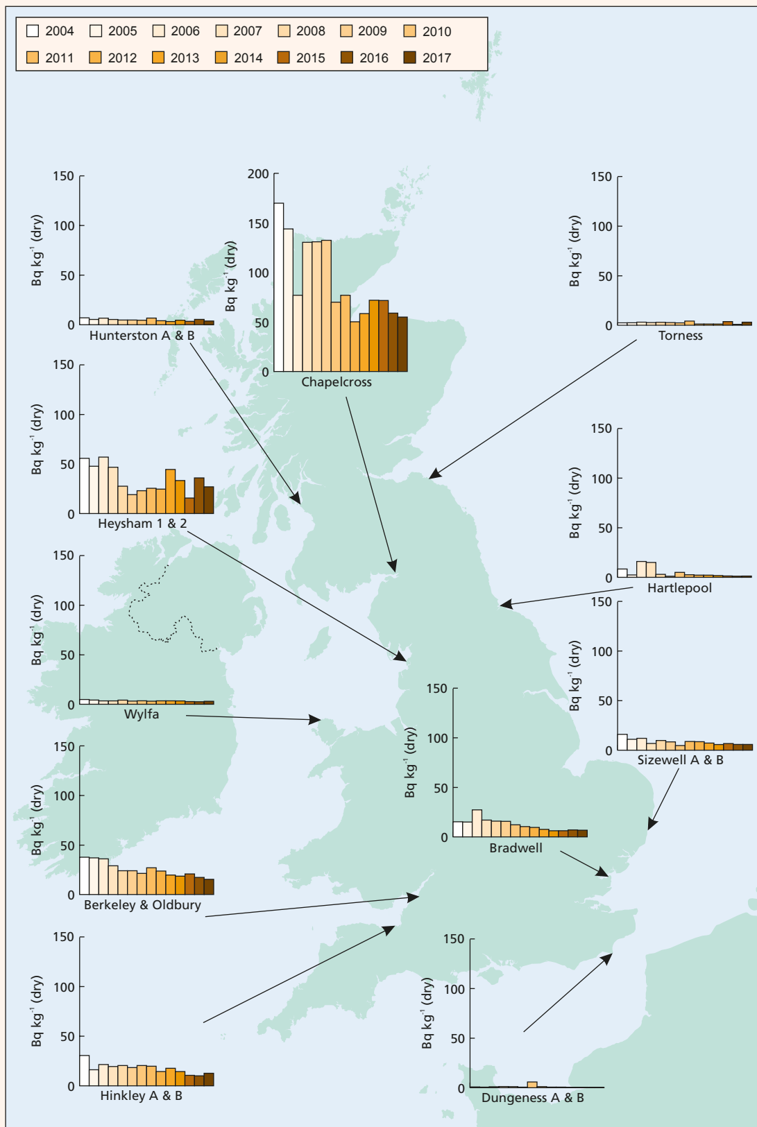
Figure 4.2. Caesium-137 concentration in marine sediments near nuclear power stations between 2004-2017
