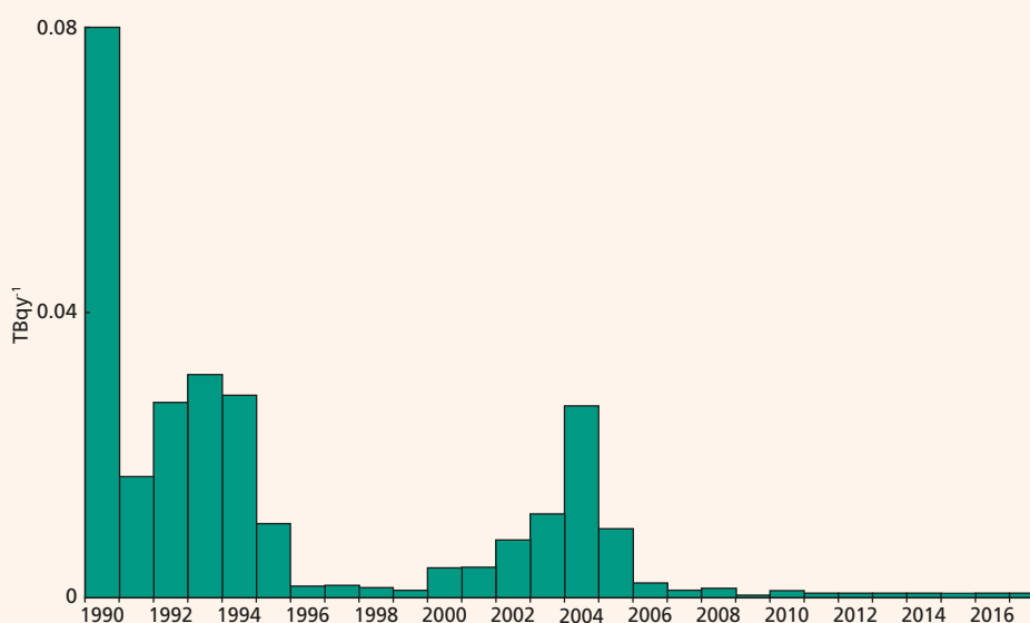
Figure 5.1. Trends in liquid discharges of tritium from Aldermaston, Berkshire 1990-2017 (including discharges to River Thames at Pangbourne, Silchester sewer and Aldermaston Stream)
