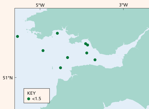
Figure 8.7. Concentrations ( \text{Bq l}^{-1} ) of tritium in surface water from the Bristol Channel, September 2017
