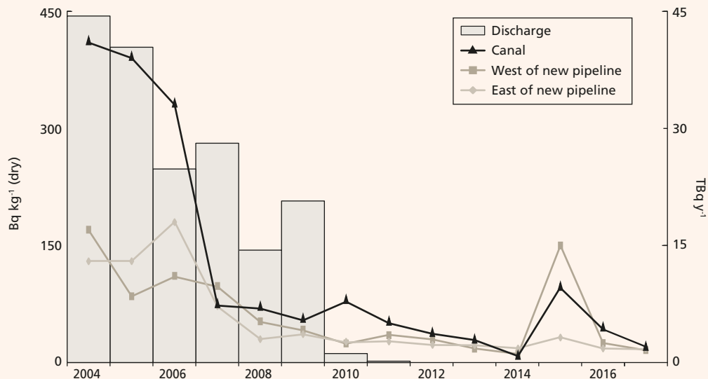
Figure 6.3. Tritium liquid discharge from Cardiff and mean concentrations in sediment near Cardiff, 2004-2017
