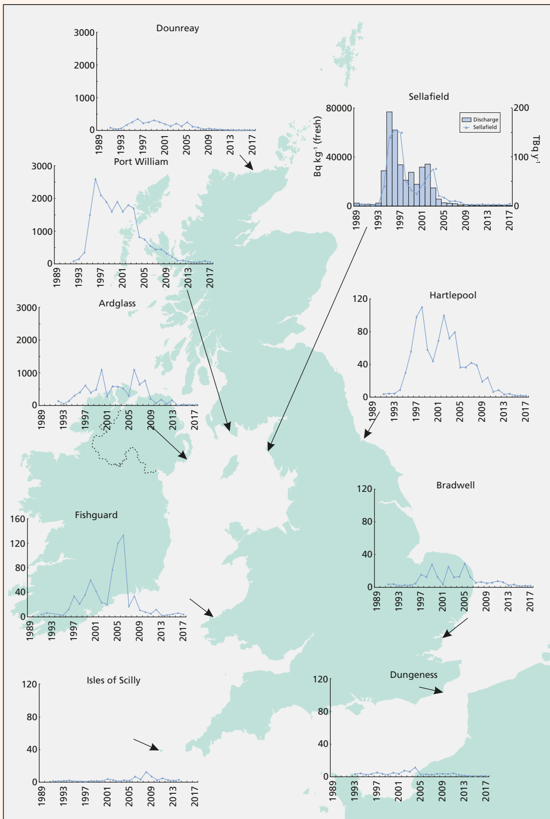
Figure 2.11. Technetium-99 in UK seaweed ( Fucus vesiculosus ) from Sellafield liquid discharges between 1989-2017 (Note different scales used for Ardglass, Doureay, Fishguard, Port William and Sellafield)
