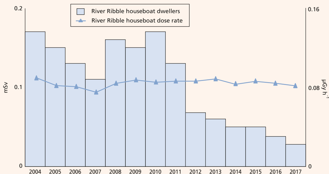
Figure 2.4. Total dose from all sources and dose rates at Springfields, 2004-2017
