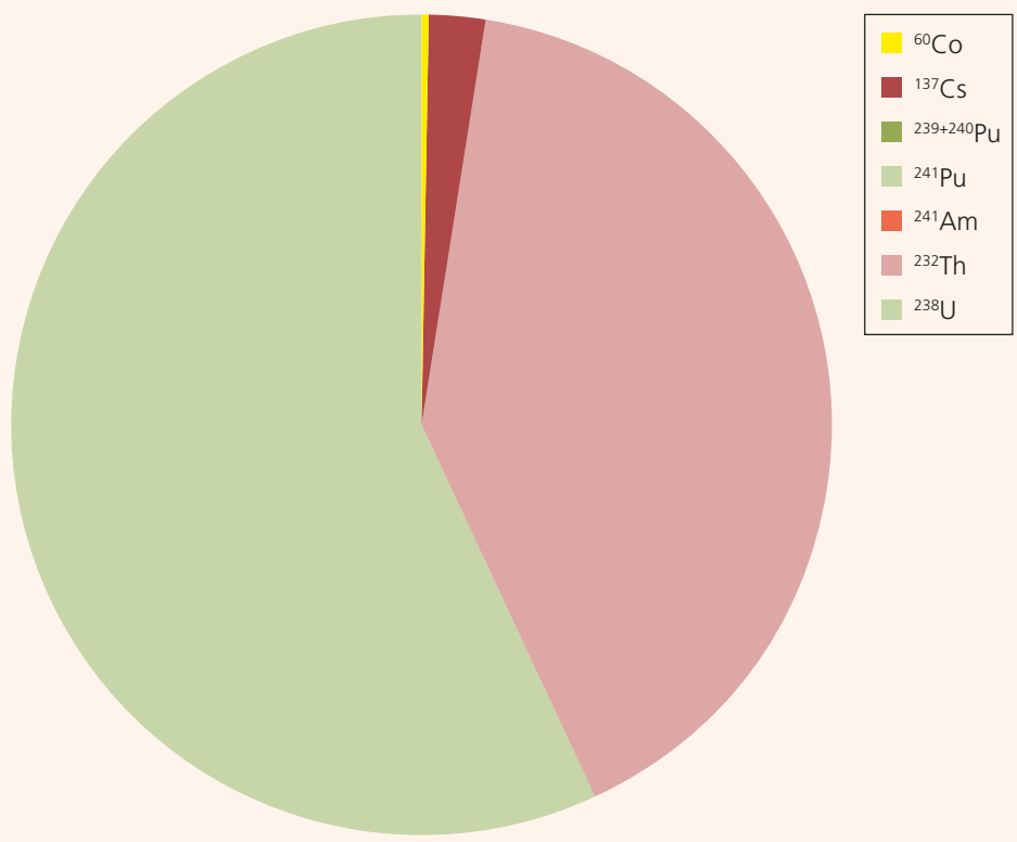
Figure A5.1. Radionuclide contribution to dose to individual crew members due to dredging at Hinkley Point C, Somerset, 2017
