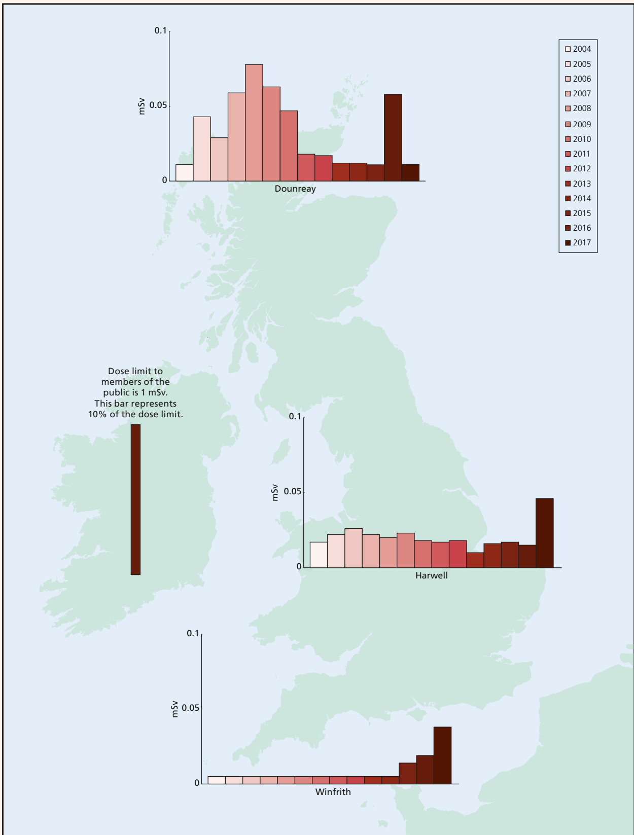
Figure 3.1. Total dose at research establishments, 2004–2017 (Small doses less than or equal to 0.005 mSv are recorded as being 0.005 mSv)
