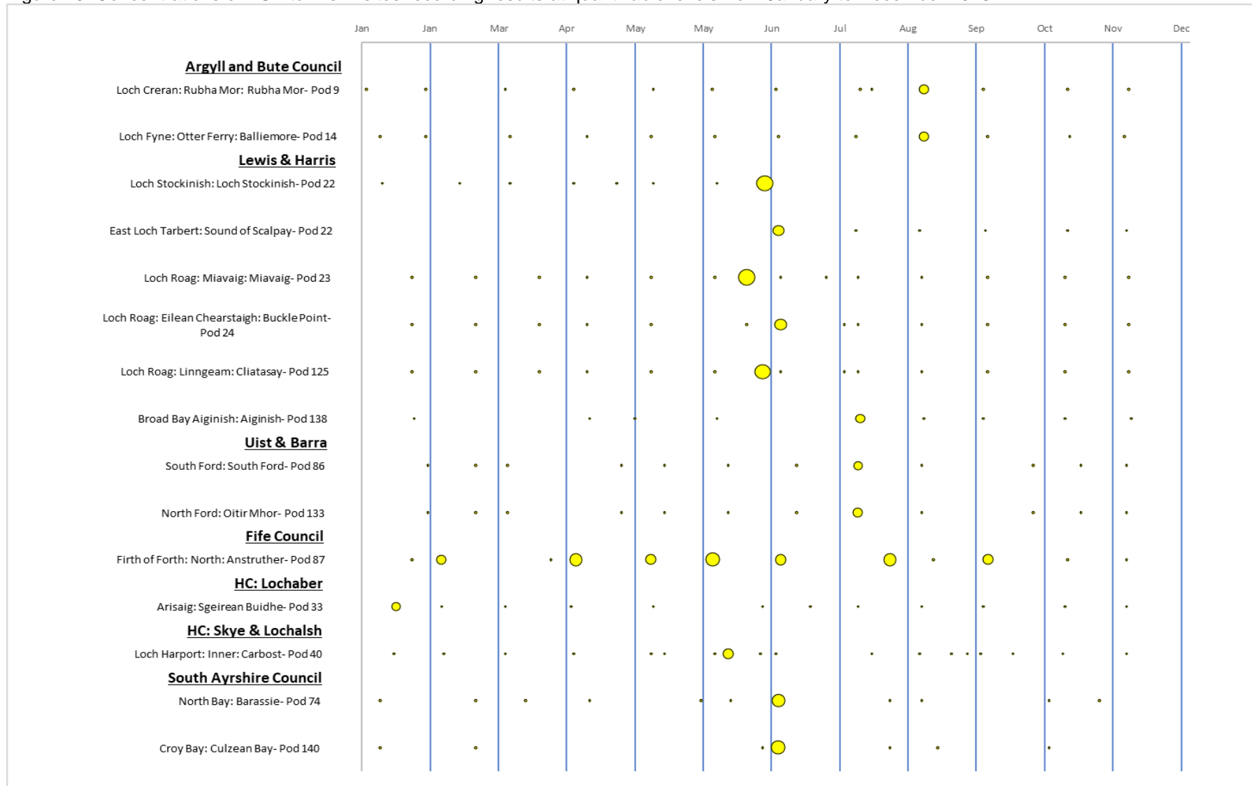
Figure 20. Concentrations of ASP toxins in sites recording results at quantifiable levels from January to December 2018
